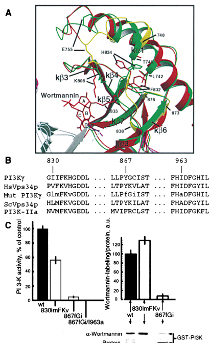
Figure 6. Wortmannin Inhibition of PI 3-Kinase
