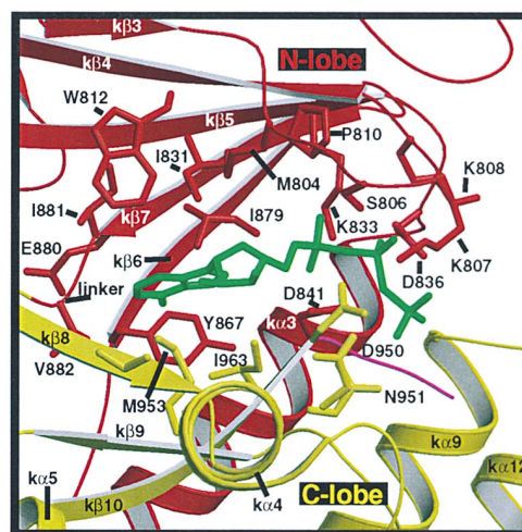
Figure 2. The ATP Binding Site of PI3Kγ
