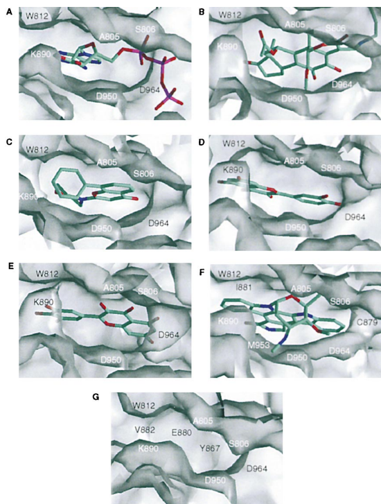
Figure 3. Interactions between Inhibitors and the PI3K Active Site. Each of the complexes was superimposed on the ATP/enzyme complex using the \alpha -carbons of the N-terminal lobe. The molecular surfaces of the enzymes are shown. The complexes represented are PI3K with (A) ATP, (B) wortmannin, (C) LY294002, (D) quercetin, (E) myricetin, and (F) staurosporine. (G) The free human PI3K active site is illustrated.
