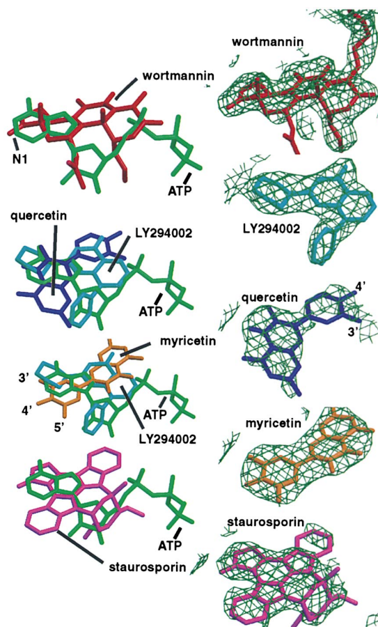
Figure 4. A Comparison of Binding Modes in the PI3K \gamma Active Site. The inhibitor/enzyme complexes were superimposed on the ATP/enzyme complex using the \alpha -carbons of the N-terminal lobe of the catalytic domain. On the left, the inhibitors are shown superimposed on ATP (green). The region of the 2mF o -DF c electron density maps for each of the compounds is illustrated on the right.
